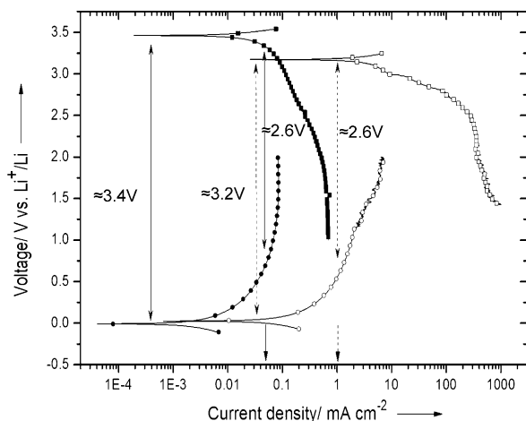
Figure 1. Potentiodynamic polarization plot obtained in (PEO) 20 LiTf electrolyte (bold black) and 1M LiTf/triglyme (black) at a scan rate of 20 mVs -1 from air electrode (rectangular) and lithium metal (circle) at 80°C and room temperature, respectively.
