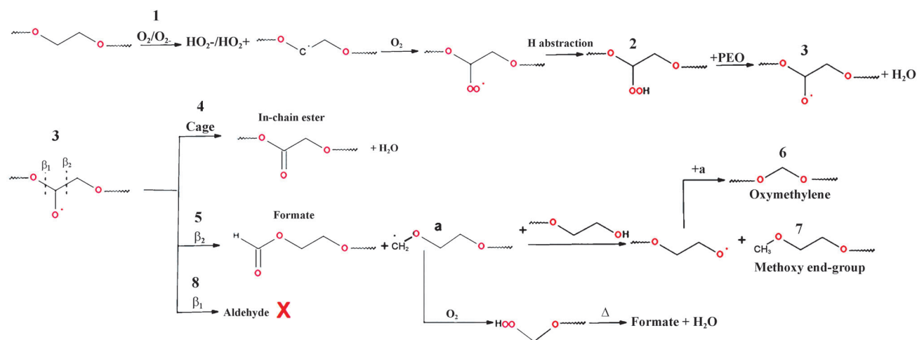
Scheme 2. Proposed mechanism for degraded \text{P}(\text{EO})_{20}\text{LiTf} electrolyte after discharged in a \text{Li}-\text{O}_2 cell at 0.05\text{ mA cm}^{-2} .
