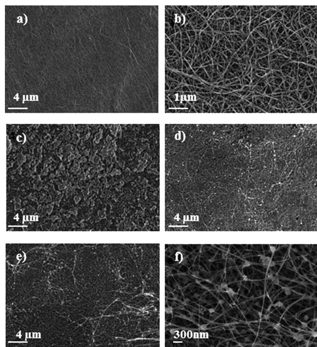
Figure 3. High-resolution SEM images of a,b) the pristine CNT air-cathode, c) the CNT air-cathode after discharged in a SPE-based \text{Li}-\text{O}_2 cell at 0.1 \text{ mA cm}^{-2} to 2.2 V acquired at the side facing the polymer electrolyte, d) after peeling about 10 \mu\text{m} of the CNT cathode, and e,f) after peeling about 20 \mu\text{m} of the CNT cathode.
