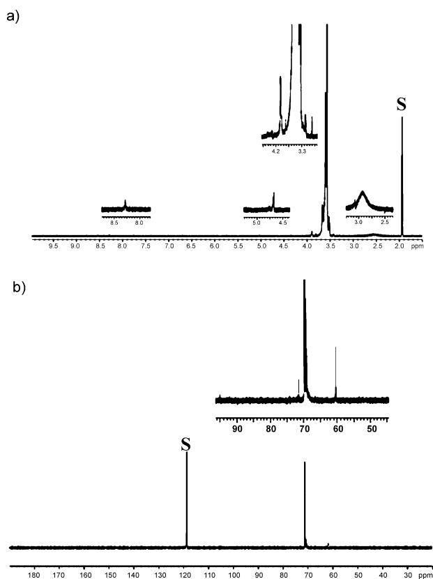
Figure 4. a) ^1\text{H} NMR spectrum of SPE after discharge at 0.05\text{ mA cm}^{-2} to 2.2 V at 80^\circ\text{C} . Expansion of the 2.5–3.0, 3.3–4.2, 4.5–5.0, 8–8.5 ppm regions are presented. b) ^{13}\text{C} NMR spectrum of SPE after discharge at 0.05\text{ mA cm}^{-2} to 2.2 V at 80^\circ\text{C} . Expansion of the 45–96 ppm region is presented. The peaks labelled by S indicates the solvent peak.
